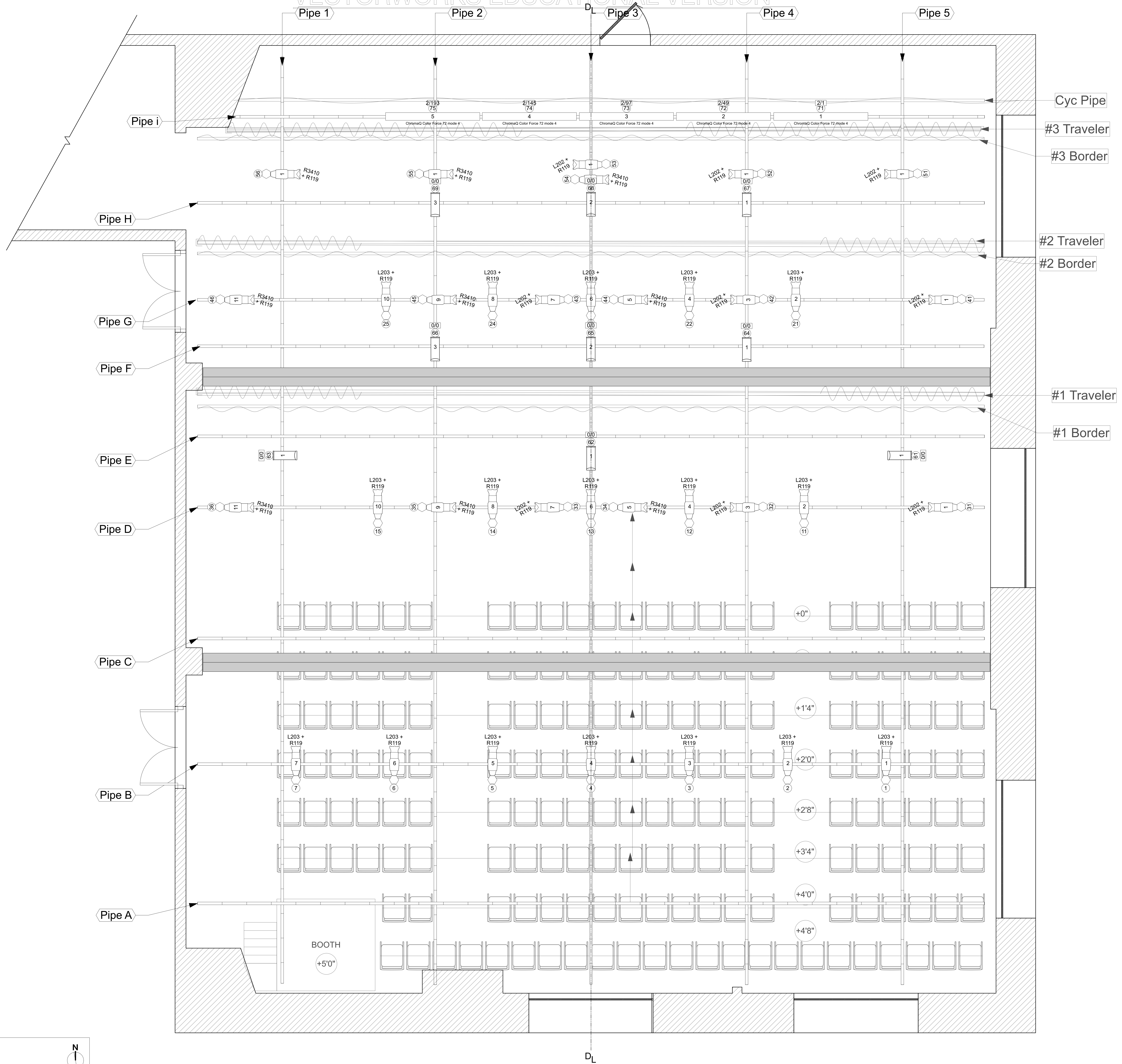
1 Auditorium Rep Plot Scale: 1/2" = 1'-0"
